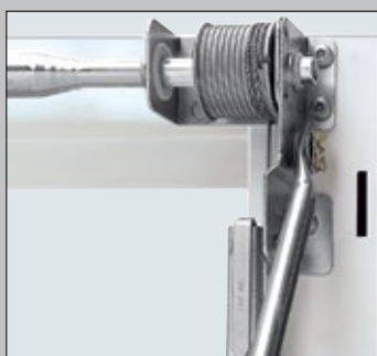
1 Cable drum
